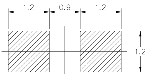
Recommend Pad Layout
