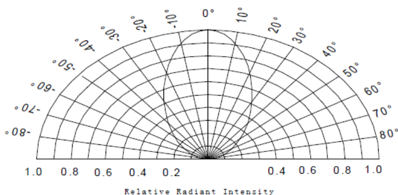
Fig.7 Radiation diagram
