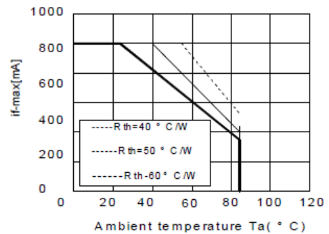
Fig.6 Maximum Driving Forward DC Current vs. Ambient Temperature (Derating based on T_J max. = 115^{\circ}\text{C} )
