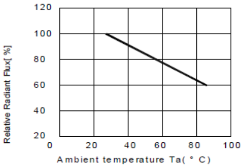
Fig.5 Relative Radiant Flux (@ 350mA) vs. Ambient temperature
